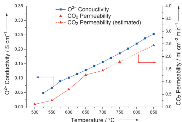
Figure 3. Temperature dependence of CO 2 permeation flux through the dual-phase membrane and the total O 2− conductivity of SDC.
